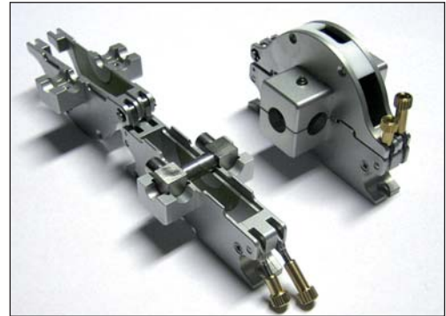
Wide Cartridge with changeable collets for standard applications except for Microfittings.
