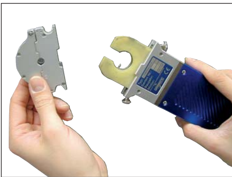
The removable cartridge system allows precise alignment of the joining parts, even under extremely narrow conditions
